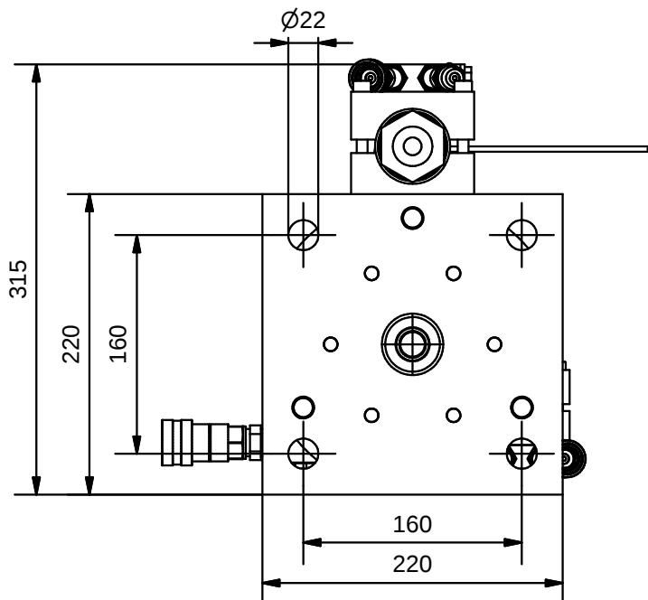
Bottom view (1:5)
